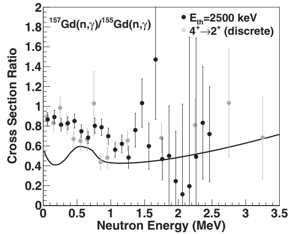
FIG. 3. The ratio of ^{157}\text{Gd}(n, \gamma)/^{155}\text{Gd}(n, \gamma) cross sections are shown for the surrogate analyses using statistical \gamma rays with E_{\text{th}} = 2.5 MeV (black points) and discrete \gamma rays using the results for 4^+ \rightarrow 2^+ transitions [20] (gray points). The smooth curve is the cross-section ratio that is calculated using reaction theory [20,25].
